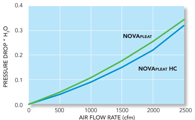
Test data results based on 24" x 24" x 2" filter sample.
